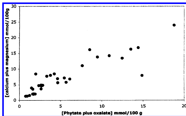
Figure 2. Correlation between phytate plus oxalate with calcium plus magnesium on molar basis in 30 soy foods ( r = 0.90 ; P < 0.001 ).
